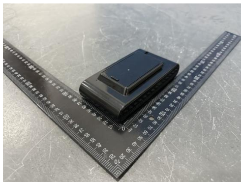
电池/ Battery (Battery Li-01 22,2V 2000mAh 44,4Wh)
